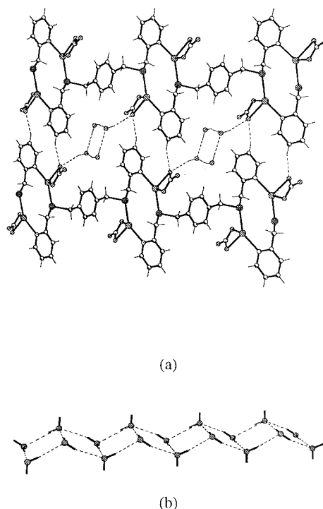
Fig. 2 (a) A view of two adjacent chains of complex 1 showing weak C(pyridine)–H⋯ONO 2 − and strong HO–H⋯ONO 2 − interactions and the corrugated ladders of water molecules running into the page. (b) View along a corrugated ladder of water molecules.
